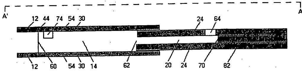
Cross Section Along A-A' of FIG. 1
